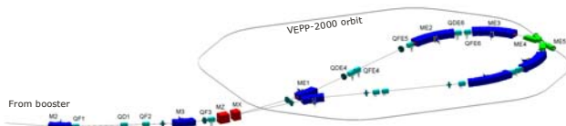
Figure 1: General view of VEPP-2000 injection channels.
