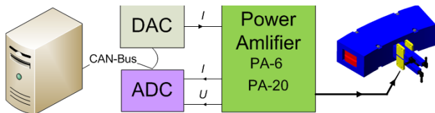
Figure 3: Steering coils supplying schematic.
