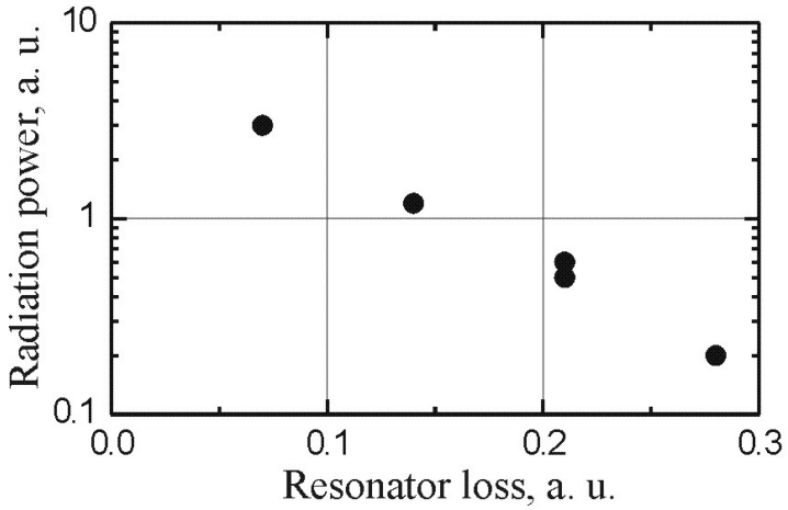
Figure 6. Average intra-cavity power vs loss per one amplification.
