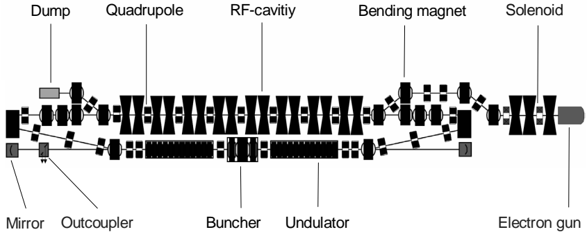
Fig. 1. Scheme of the first stage of Novosibirsk high power free electron laser.
