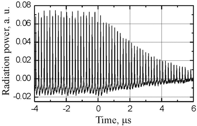
Figure 4. Time history of the output radiation power after switching the electron beam off.
