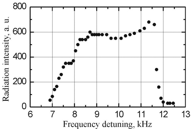
Figure 2. Laser intensity vs RF frequency detuning ( f\theta - 180400 kHz).
