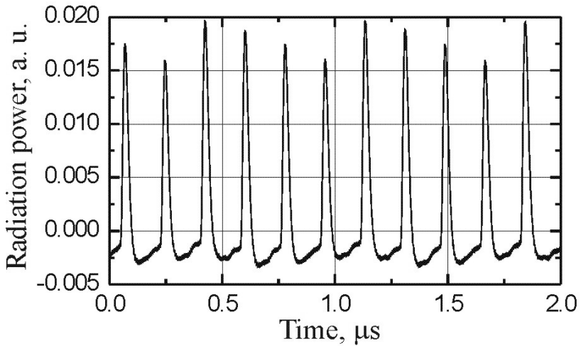
Figure 5. The output radiation time dependence; electron bunch repetition rate 1.4 MHz is four time less then the optical resonator round-trip frequency 5.6 MHz.
