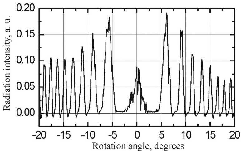
Figure 3. Results of the Fabri-Perot interferometer rotation angle scanning (laser wavelength \lambda = 136\mu\text{m} ).
