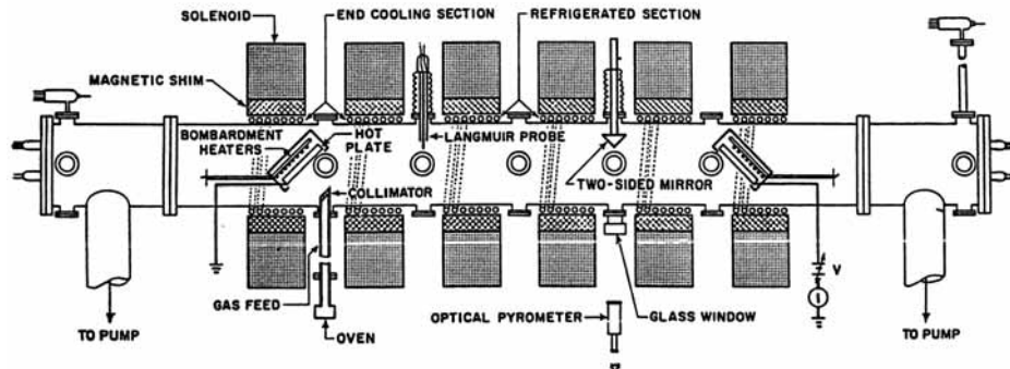
Fig. 6. Diagram of the Q machine, showing the solenoids that produce the axial magnetic-confinement field and the two hot tungsten plates mounted at 45 degrees for the production of alkali-metal plasmas. Source: N. Rynn, "Plasma Column End Effects," in Pardo and Robertson, Plasma Instabilities and Anomalous Transport (ref. 53), p. 107.
