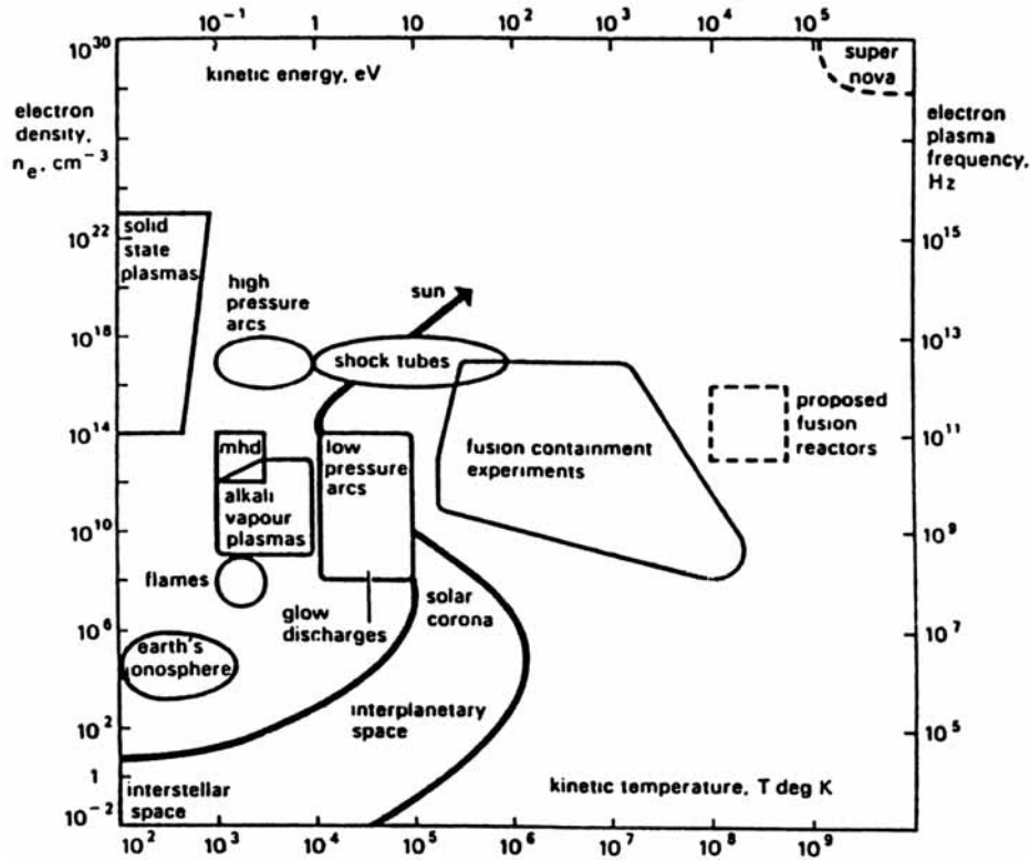
Fig. 4. A variant of the Kantrowitz-Petschek map, showing various plasma regimes, including those pertaining to space and astrophysical plasmas, gaseous electronics, and fusion research, against logarithmic scales of electron density and kinetic temperature. Source: Physics Survey Committee, Physics in Perspective (ref. 95), p. 219.
