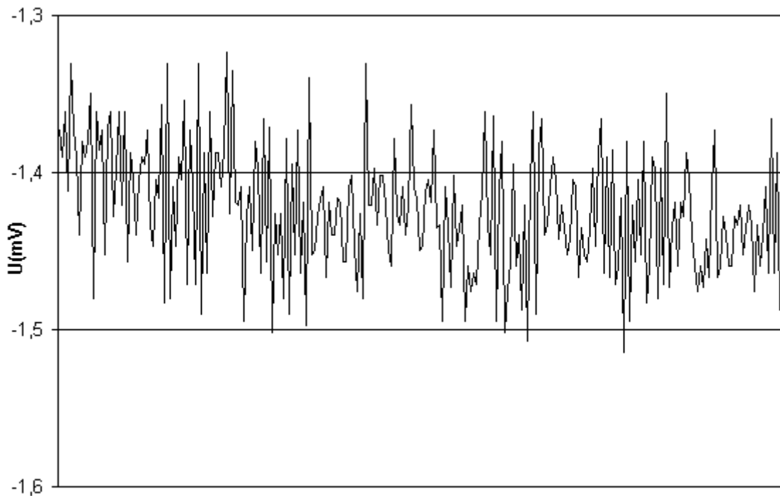
A typical noise of ADC. A data were collected in single-channel mode, data rate was 1 ms/measurement.
