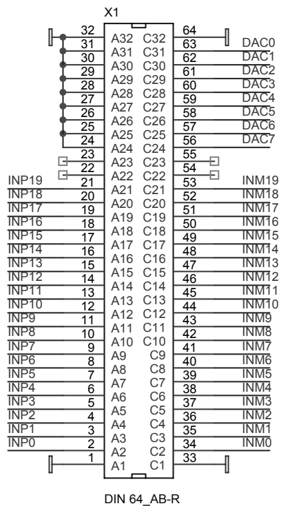
Pinout of X1 for CEAC208.
