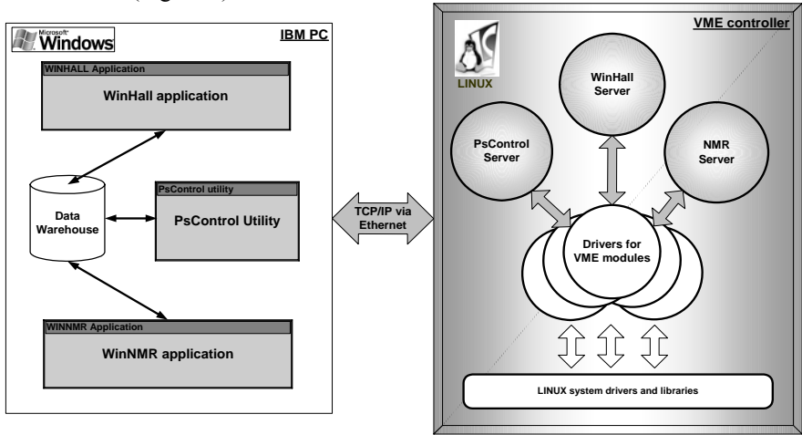
Figure 4. Architecture of software of Hall measuring system
