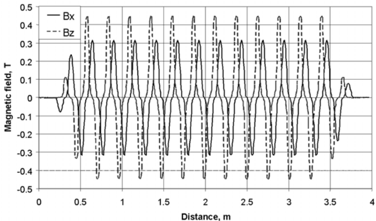
Figure 7. HU256 magnetic field map
