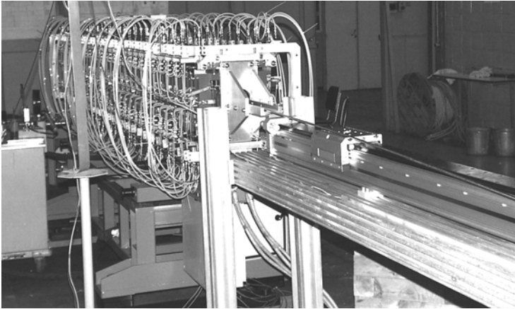
Figure 6. View of undulator and measuring assembly
