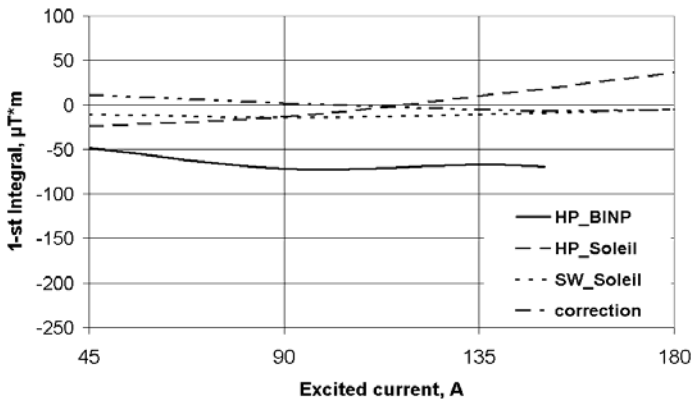
Figure 8. HU256 first integral vs. current
