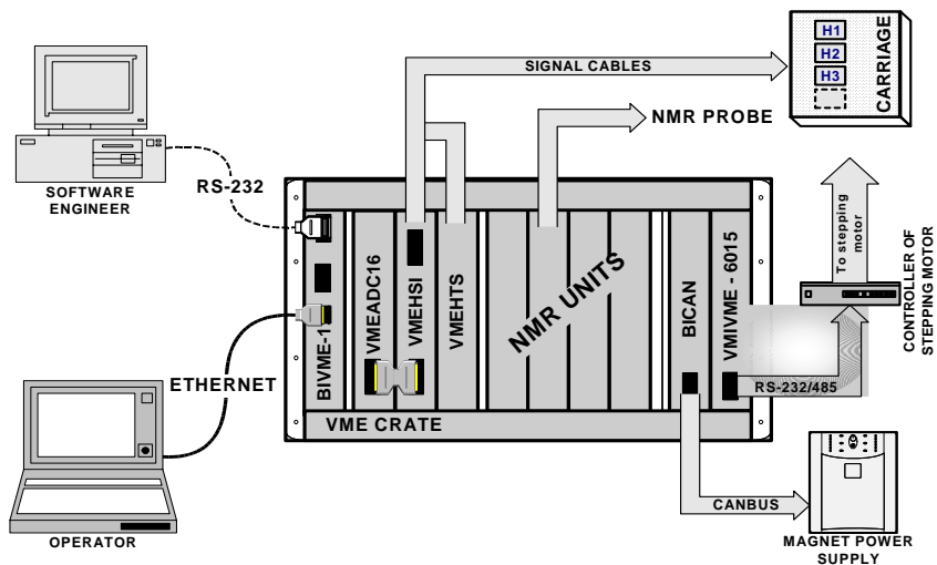
Figure 1. The structure of Hall measuring system.
