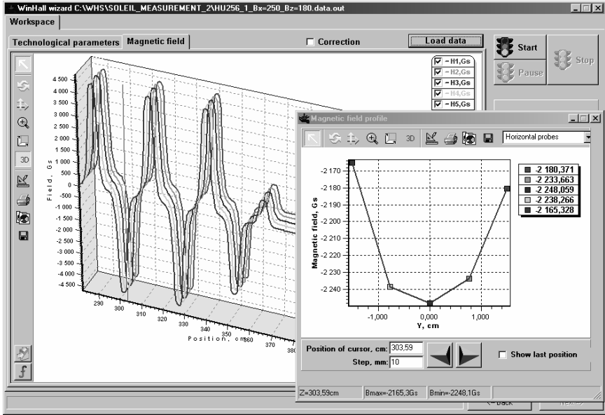
Figure 5. View of operator's main window of WinHall program and demonstration of visualization of measured data
