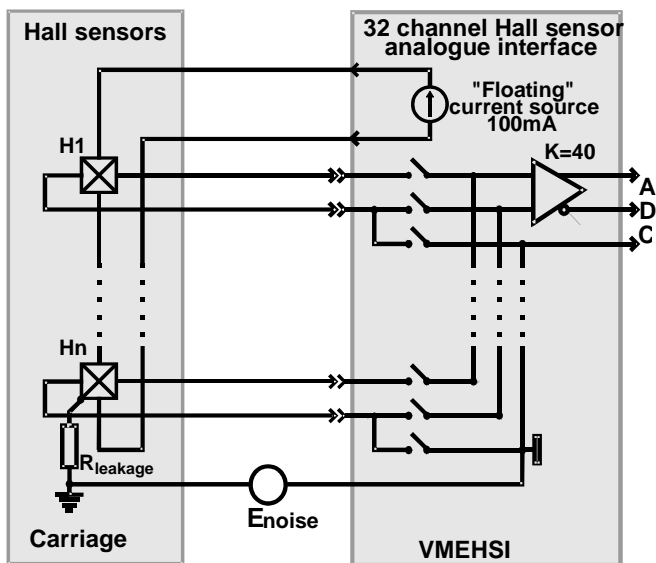
Figure 3. The structure of VMEHSI and its connections to Hall sensor carriage
