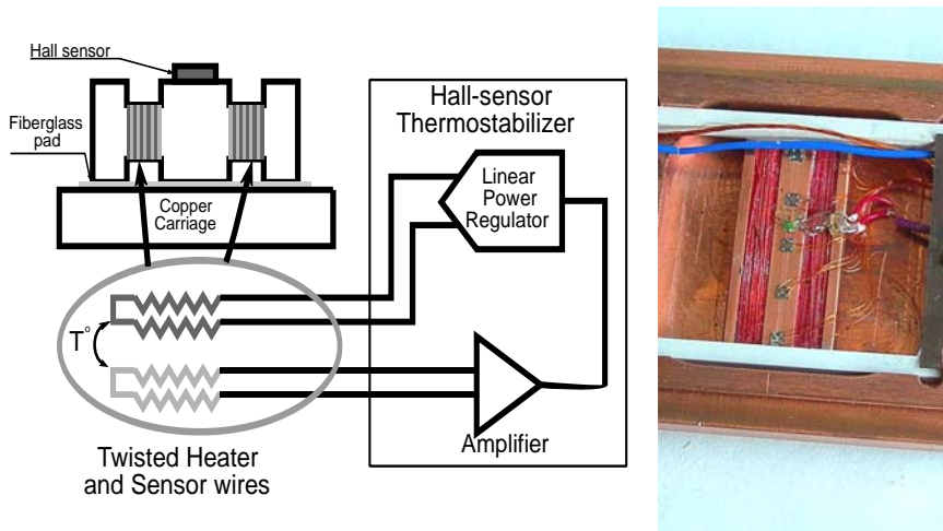
Figure 2. Principles of sensors thermostabilization and view of sensors, installed on thermostabilized holder
